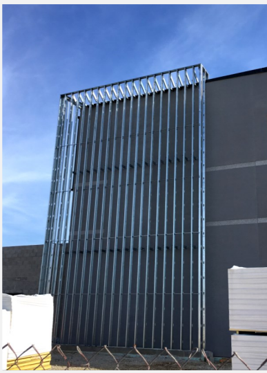
Gym Metal Panel Framing—West Elevation
